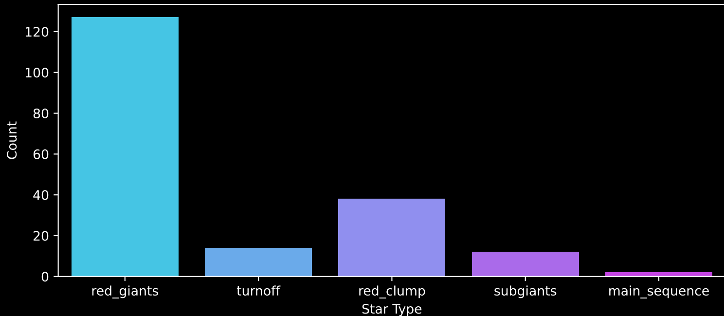
APOGEE DR17 Field: [COROTA2-RV] Count plot of Star Type
