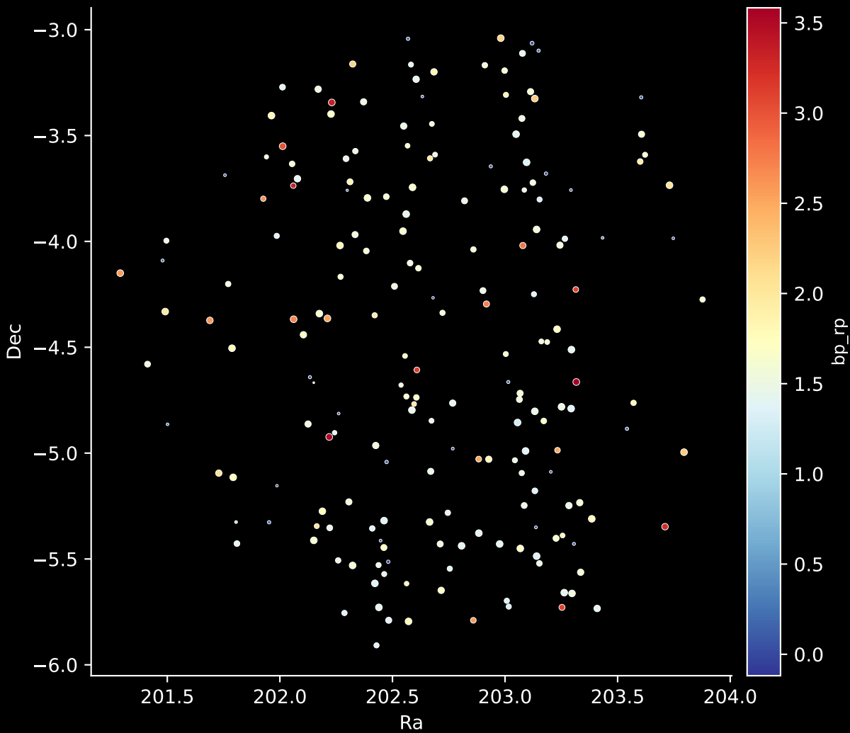
APOGEE DR17 Field: [COROTA2-RV] Stars: 193
