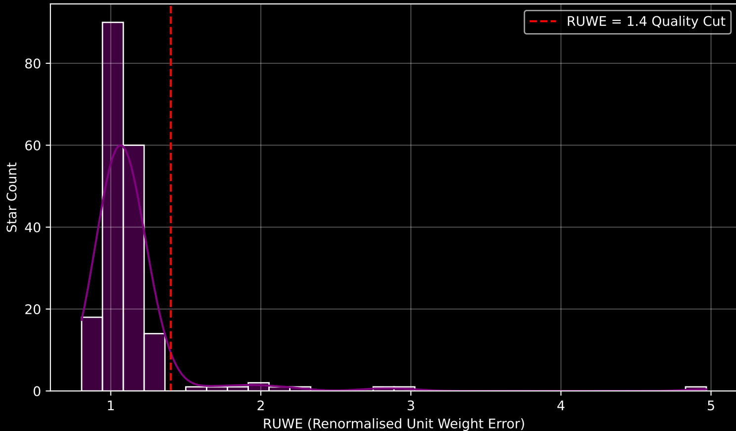
GAPOGEE DR17 Field [COROTA2-RV] RUWE Distribution (n= 192)
