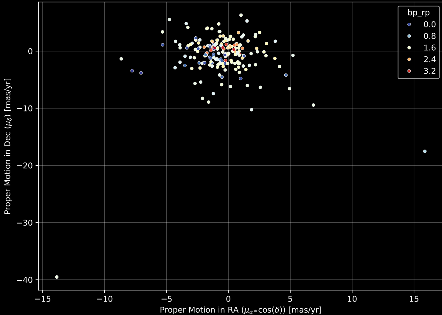
APOGEE DR17 Field: [COROTA2-RV] Proper Motion Diagram (n= 193)
