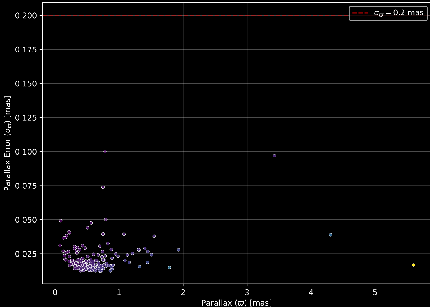
APOGEE DR17 Field: [COROTA2-RV] Parallax Quality (n= 193)
