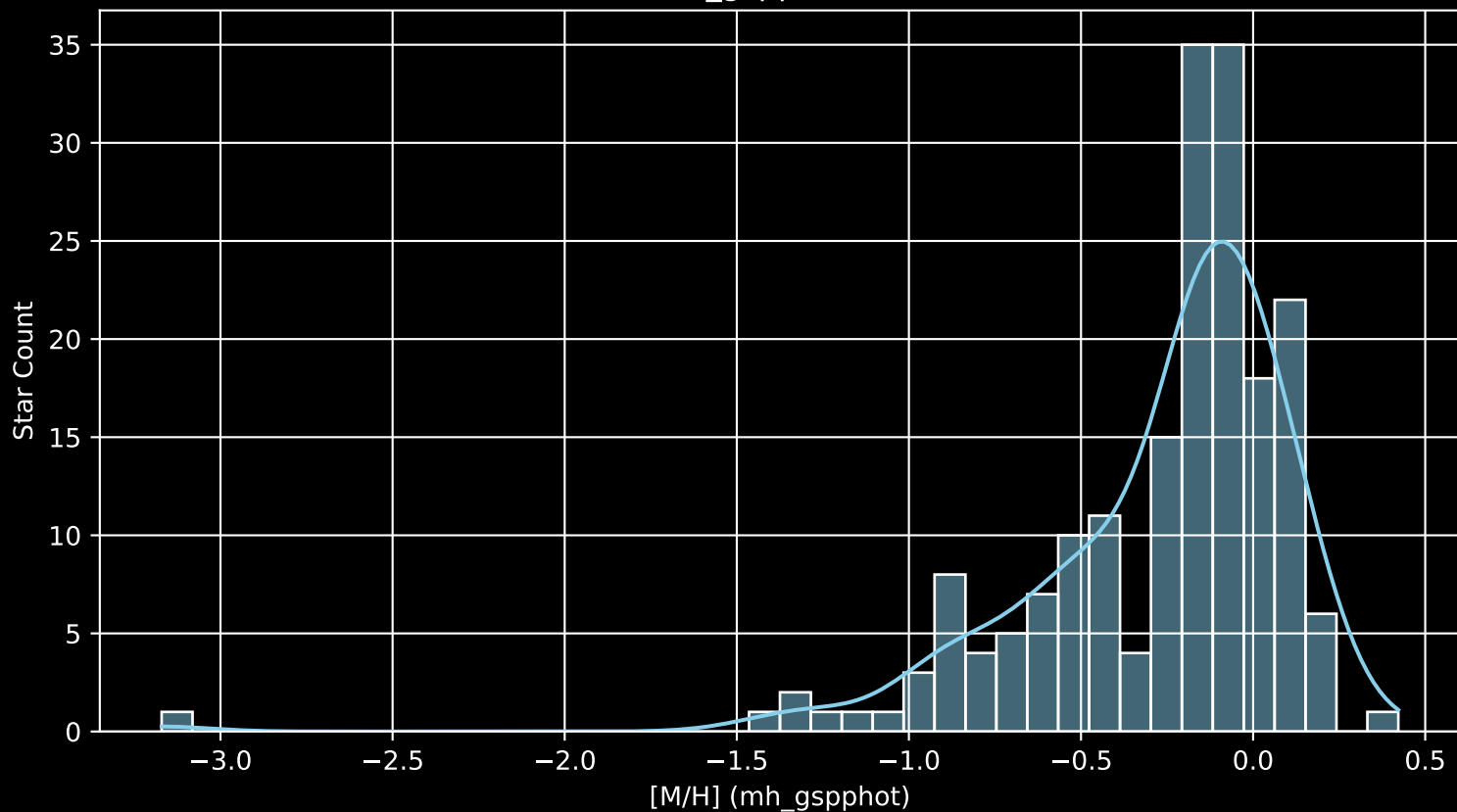
APOGEE DR17 Field: [COROTA2-RV [M/H] (mh_gspphot) (n= 191)
