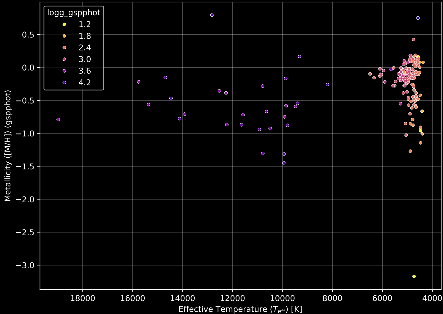
APOGEE DR17 Field: [COROTA2-RV] Stellar Population Parameters (n= 193)
